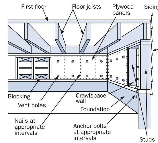
Figure A. Strengthening weak crawlspace walls.
