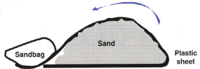
Temporary Levee -Side View
