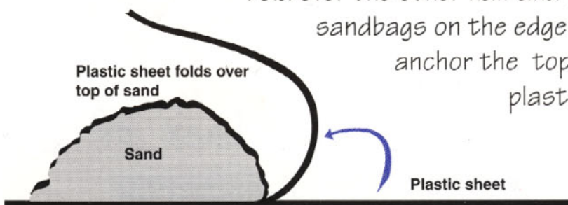
Temporary Levee -Side View
